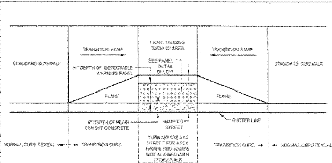
TYPICAL INSTALLATION
